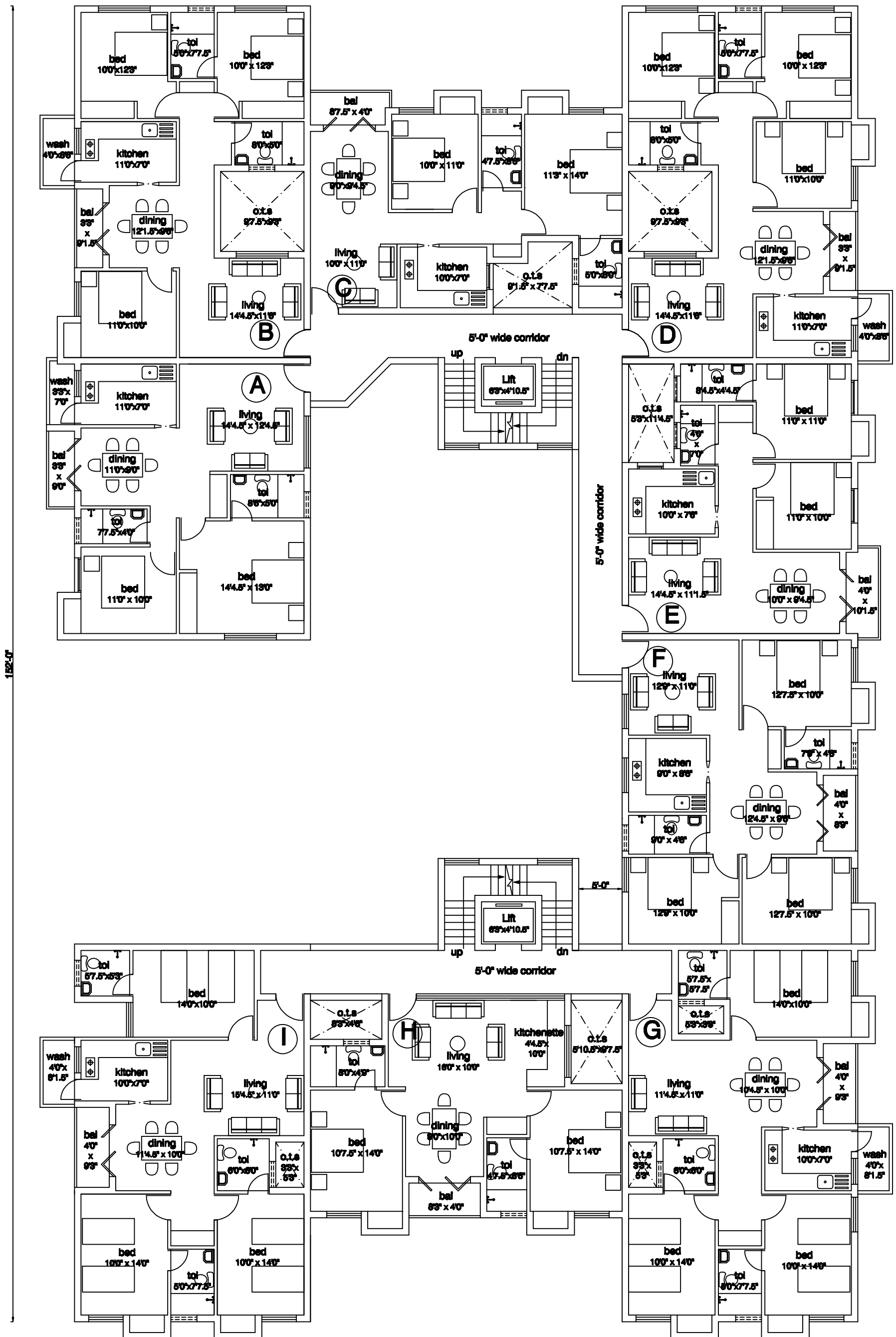
TYPICAL FLOOR PLAN (1, 2 & 3)
